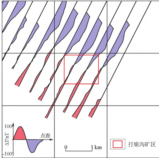
图3 打柴沟矿区1:5万地磁ΔT异常剖面平面 Fig.3 Section plan of 1:50 000 ΔT geomagnetism anomaly in Dachaigou mining area
