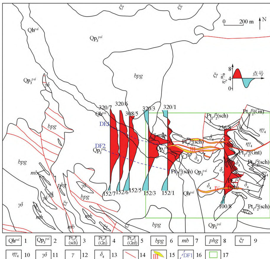
1—全新统洪冲积; 2—更新统洪冲积; 3—金水口岩群绢云石英片岩; 4—金水口岩群灰岩; 5—金水口岩群片岩夹变砂岩夹片麻岩; 6—金水口岩群灰黑色黑云斜长片麻岩; 7—金水口岩群大理岩; 8—金水口岩群灰黑色斜长角闪片麻岩; 9—正长花岗岩; 10—二长花岗岩; 11—花岗闪长岩; 12—花岗岩; 13—闪长岩; 14—断裂; 15—矿带及编号; 16—推断构造; 17—打柴沟矿区 1—Holocene alluvial sediments; 2—Pleistocene alluvial sediments; 3—sericite quartz schist of Jinshuikou group; 4—limestone of Jinshuikou group; 5—schist interbedded with metamorphic sandstone interbedded with gneiss of Jinshuikou group; 6—gray black biotite plagioclase gneiss of Jinshuikou group; 7—marble of Jinshuikou group; 8—grayish black amphibolite gneiss of Jinshuikou group; 9—syenogranite; 10—monzogranite; 11—granodiorite; 12—granite; 13—diorite; 14—fracture; 15—ore belt and number; 16—inferred structure; 17—Dachagou mine
