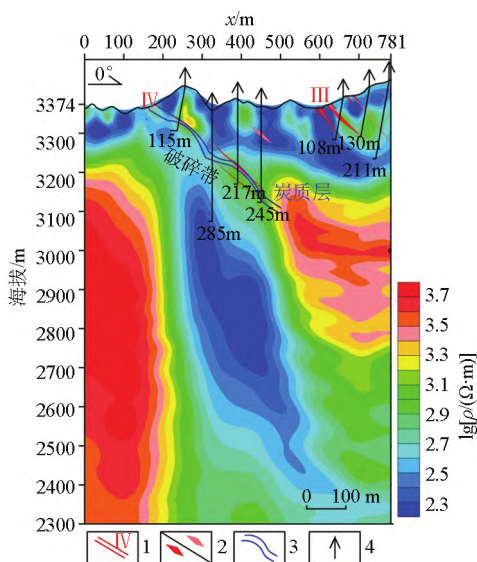
1—矿带; 2—矿体\矿化体; 3—炭质层; 4—钻孔 图 7 打柴沟 8 勘探线地质—WFEM 反演成果 Fig. 7 Geological and WFEM inversion results of Dachagou line 8
